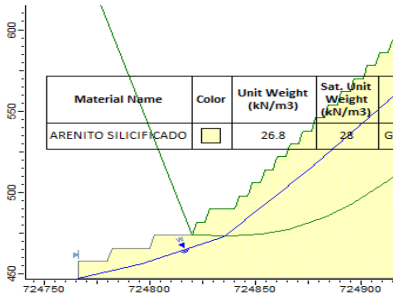
Figure 16-44 Limit-equilibrium analysis results for Section 09 with FS (safety factor) = 1.54
