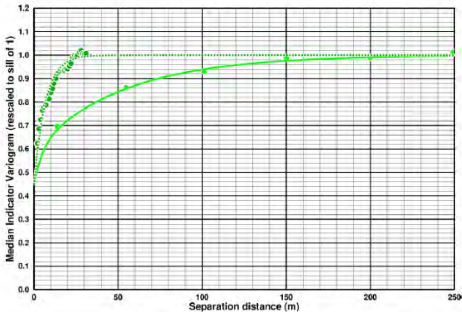
Figure 14-12 Median indicator variography for non-ferrous sediments, with the solid green line showing the omnidirectional variogram in the bedding plane and the dotted dark green line showing the variogram perpendicular to bedding.
