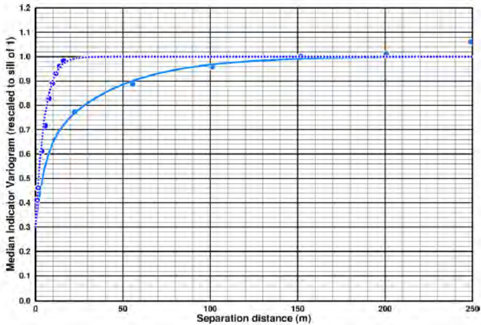
Figure 14-13 Median indicator variography for the mafic dykes, with the solid blue line showing the omnidirectional variogram in the average dip plane of the dykes and the dotted darker blue line showing the variogram perpendicular to the dykes.
