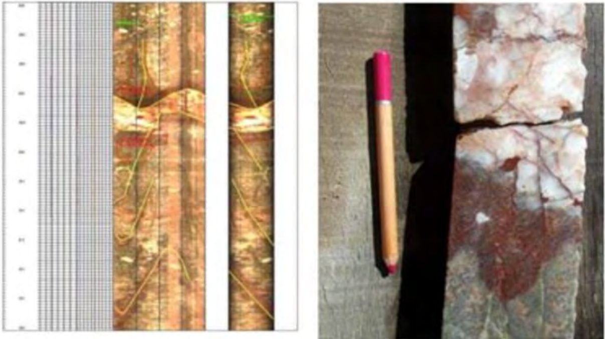
Figure 9-2 OTV image of a diamond hole compared with actual core from the same interval.
