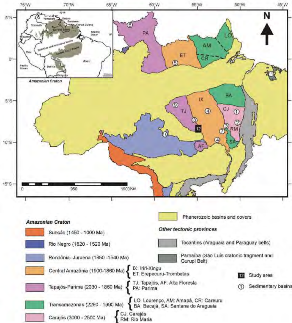
Figure 7-2 Amazonian Craton and its major geochronological domains (Source: Klein et al., 2017).
