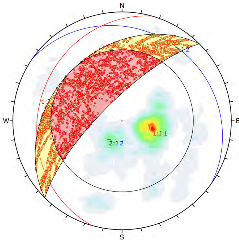
Figure 16-35 Kinematic analysis for the slope T6 showing 15% of probability for wedge rupture
