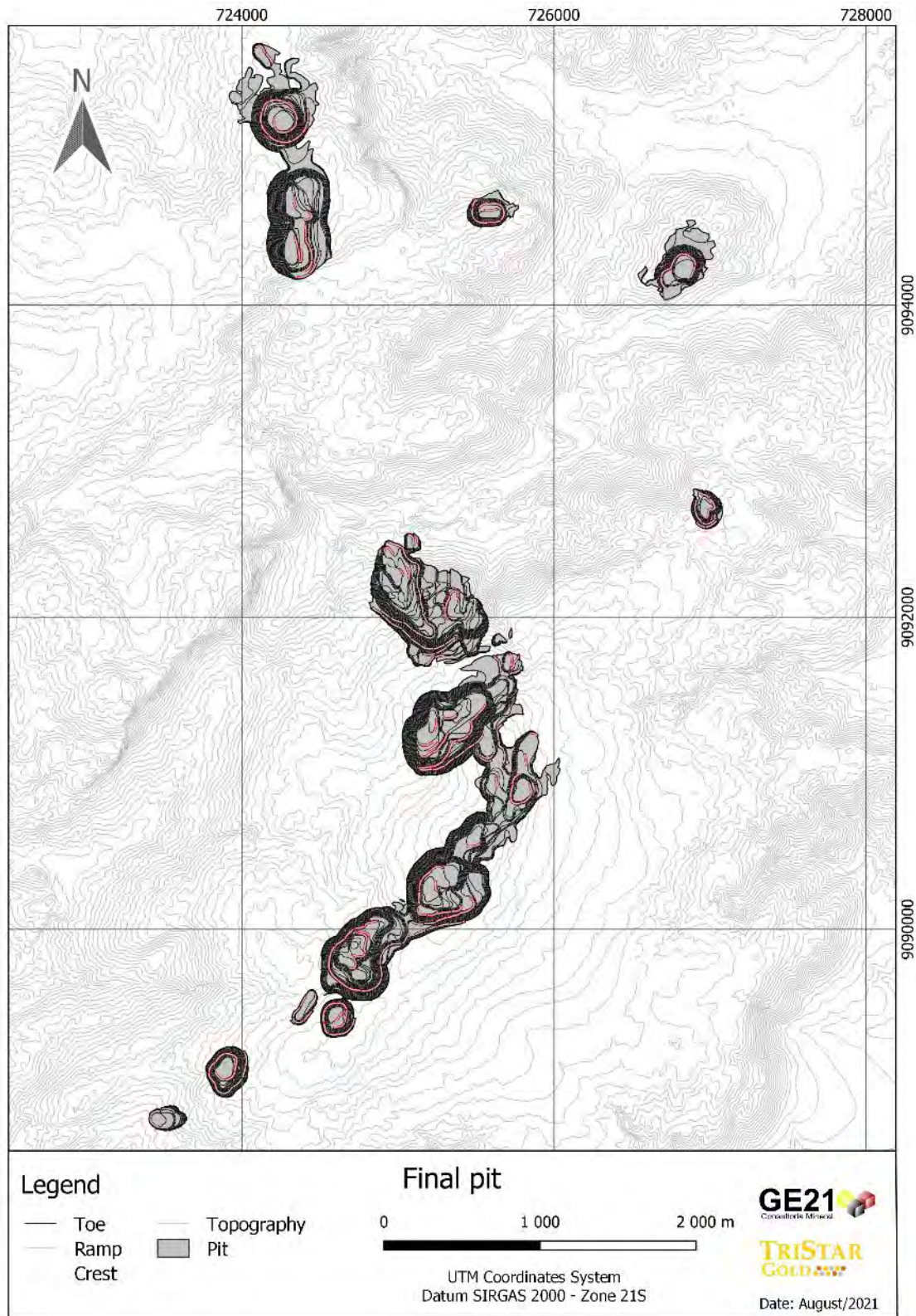
Figure 16-55 Final Pit – CDS Project
