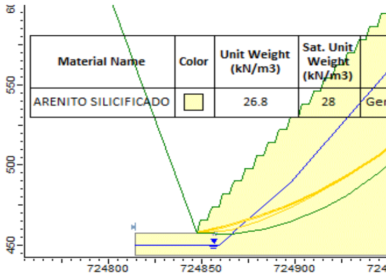
Figure 16-45 Limit-equilibrium analysis results for Section 10 with FS (safety factor) = 1.40
