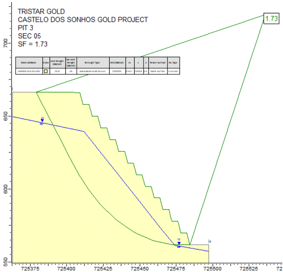
Figure 16-39 Limit-equilibrium analysis results for Section 05 with FS (safety factor) = 1.73
