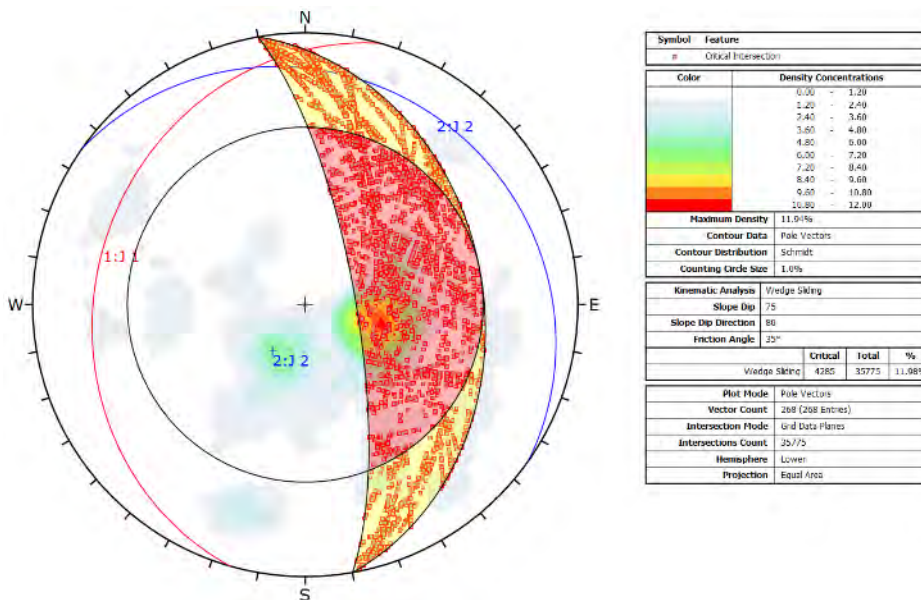
Figure 16-29 Kinematic analysis for the slope T5 showing 5% of probability for wedge rupture
