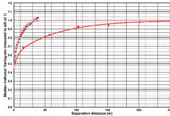
Figure 6-4 Median indicator variography for the ferrous sediments, with the red line showing the omnidirectional variogram in the bedding plane and the dotted dark red line showing the variogram perpendicular to bedding.
