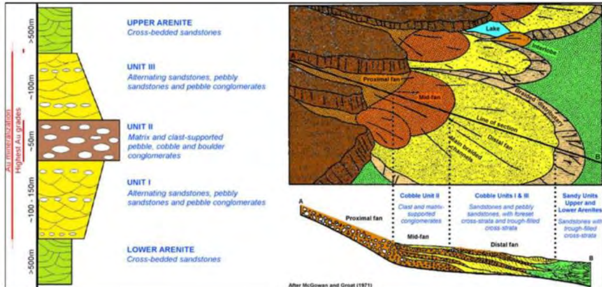
Figure 7-4 Schematic stratigraphy of the main units within the central conglomeratic band of Castelo dos Sonhos Formation, and conceptual model of the depositional environment. (Source: Modified by Karpeta, 2016, after McGowan and Groat, 1971)
