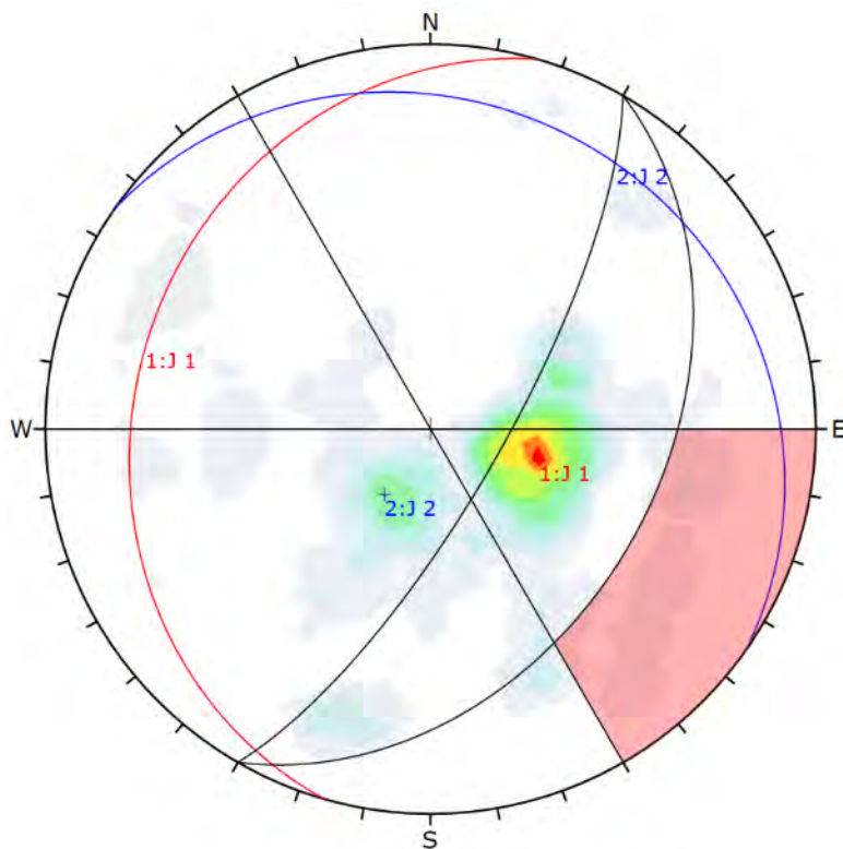
Figure 16-25 Kinematic analysis for the slope T4 showing 9% of probability for toppling rupture
