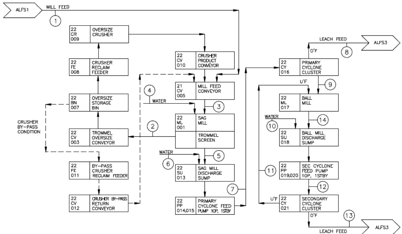
Figure 17-3 Simplified Conceptual Flowsheet – Grinding and Classification
