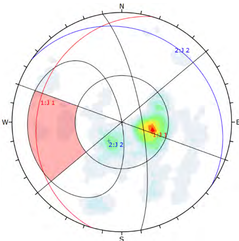
Figure 16-27 Kinematic analysis for the slope T5 showing 9% of probability for planar rupture
