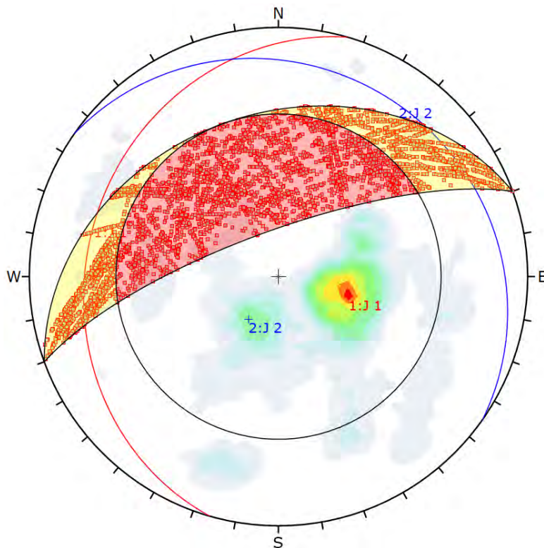
Figure 16-17 Kinematic analysis for the slope T2 showing 16% of probability for wedge rupture
