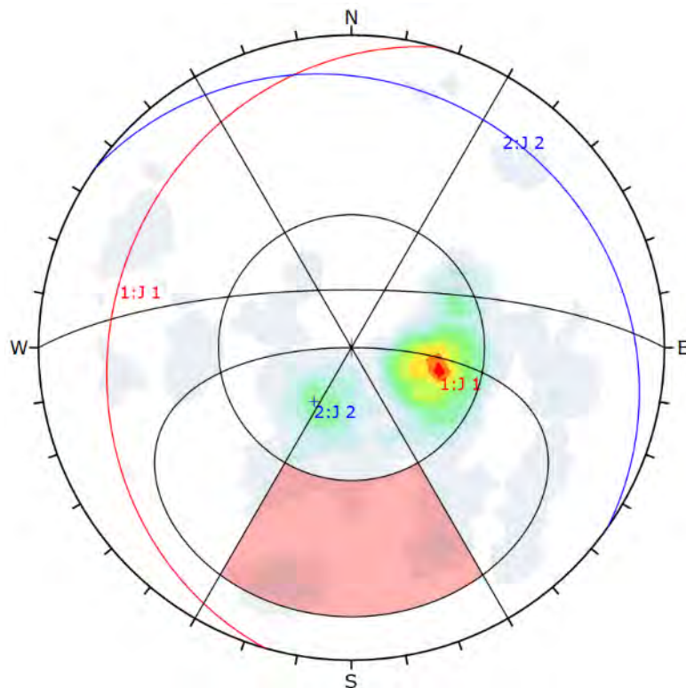
Figure 16-36 Kinematic analysis for the slope T7 showing 12% of probability for planar rupture
