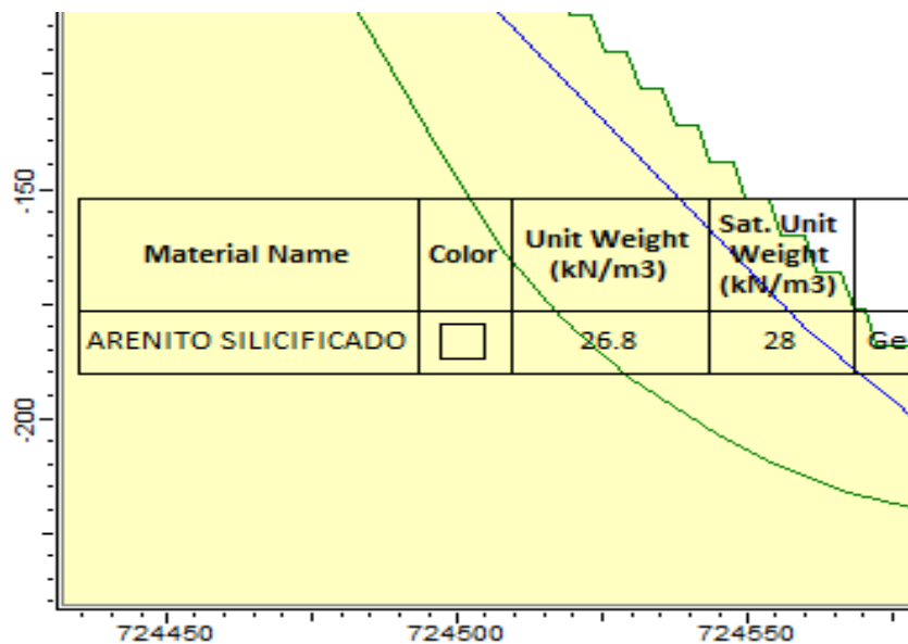
Figure 16-46 Limit-equilibrium analysis results for Section 11 with FS (safety factor) = 1.48
