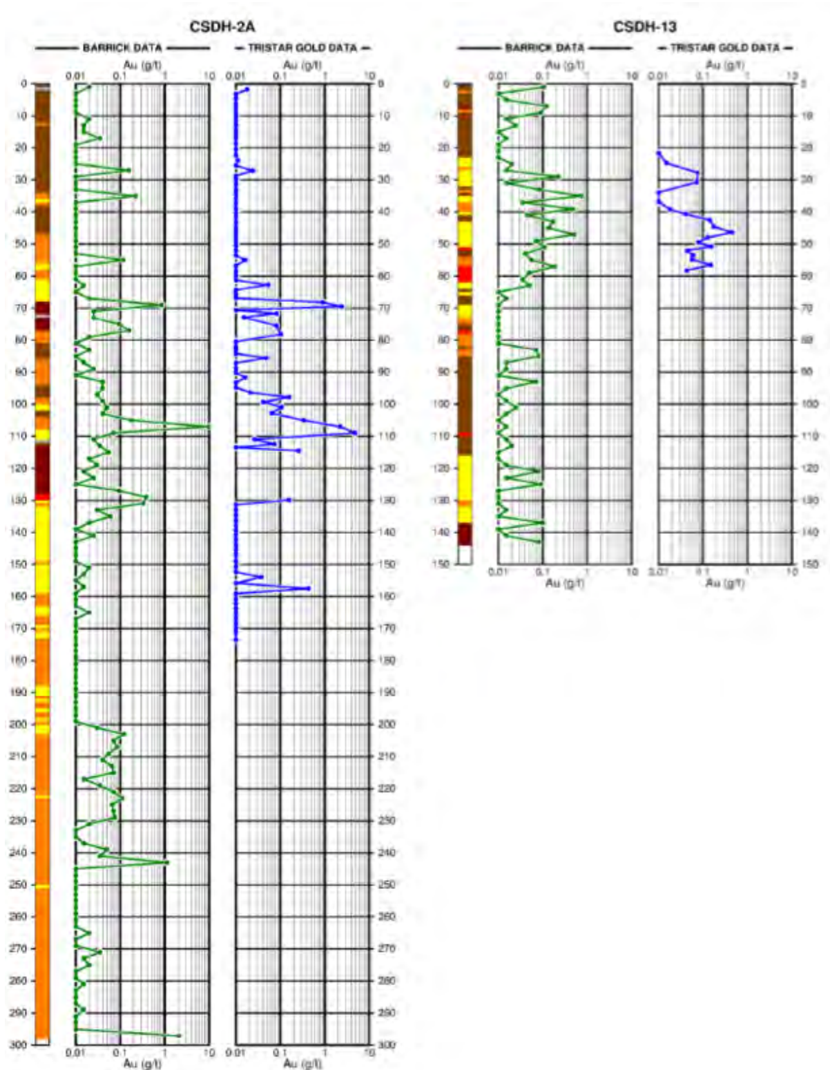
Figure 12-1 Comparison of Barrick ½-core assays to TriStar ¼-core assays, with Barrick assays having been composited to the 2m intervals sampled by TriStar.
