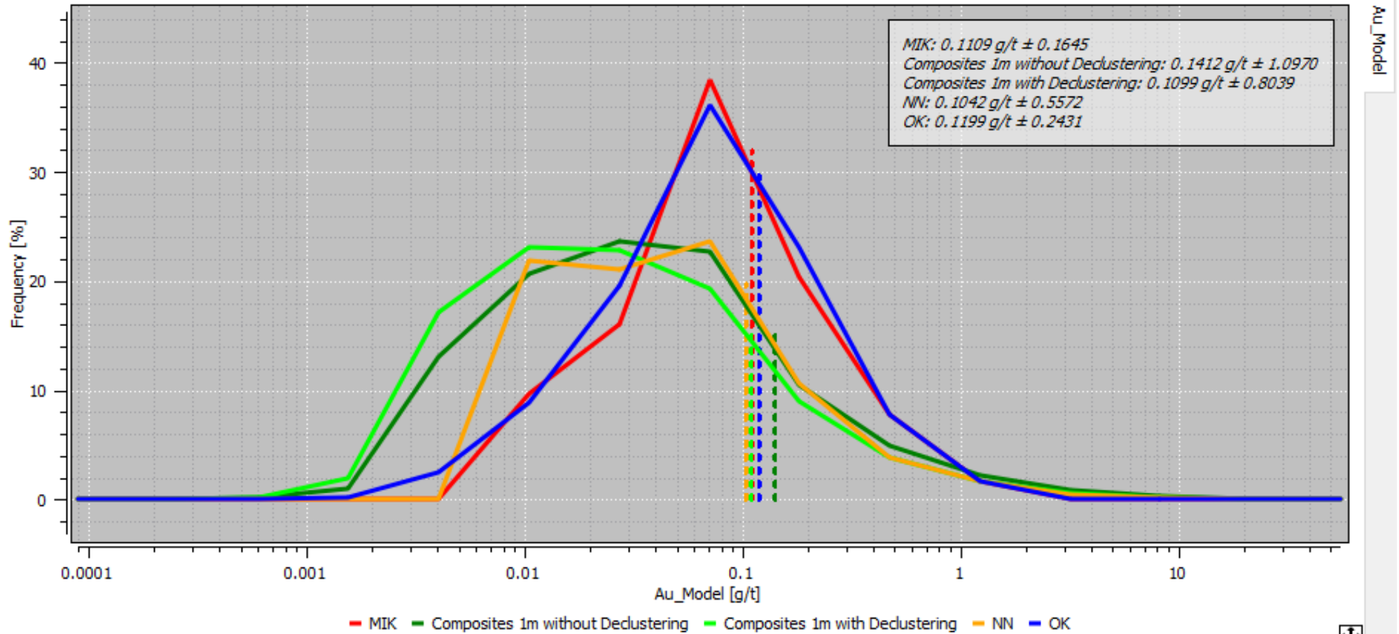
Figure 14-19 Resource validation - Esperança South region of Castelo de Sonhos - Histogram (MIK – TriStar in red, OK GE21 in blue, NN in yellow, data in green)
