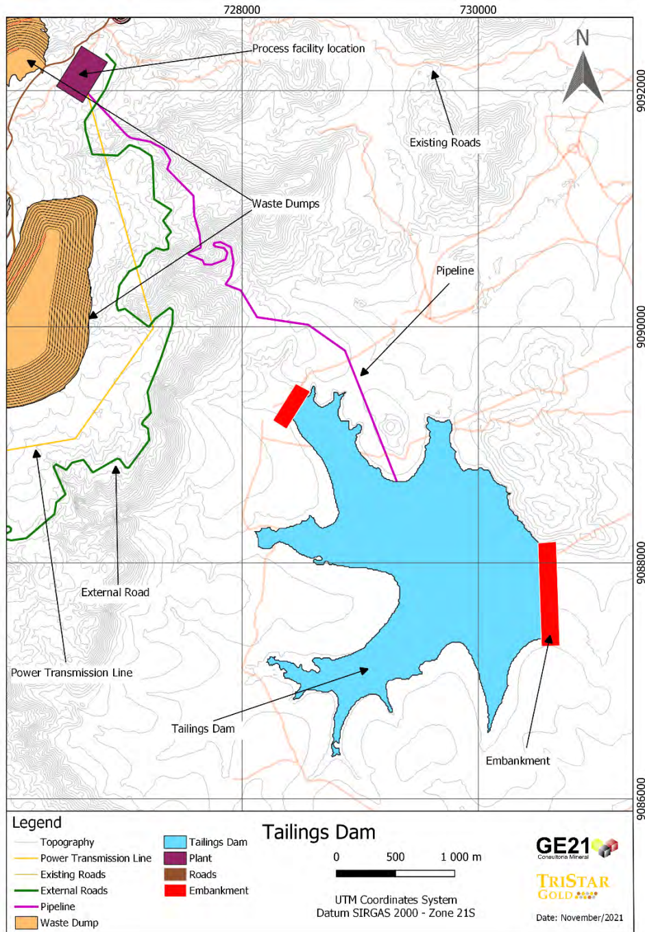
Figure 18-2: Tailing Storage Facility Design
