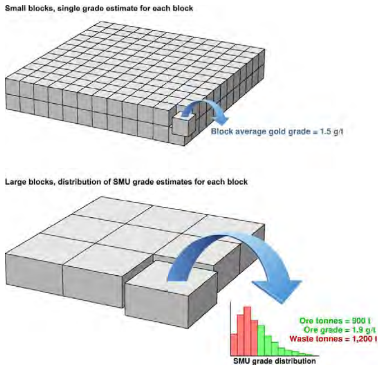
Figure 14-15 Schematic showing the difference between a conventional single-estimate block model and a recoverable-resources block model that provides an estimate of the SMU grade distributions within large blocks.
