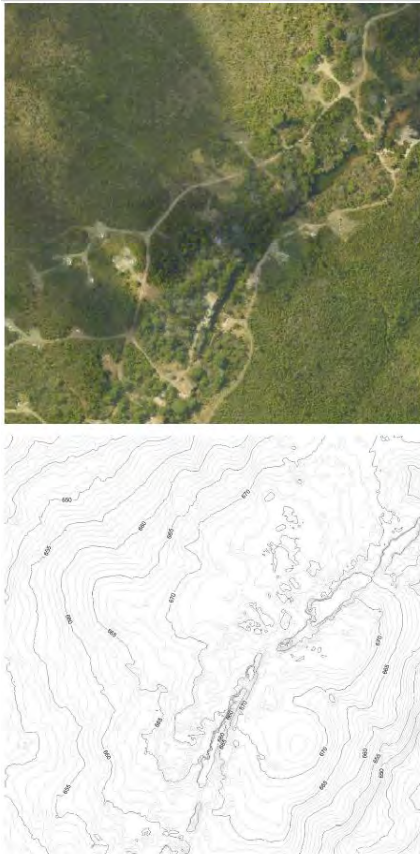
Figure 14-3 An example of the LIDAR topography's ability to identify surface depressions of garimpos.
