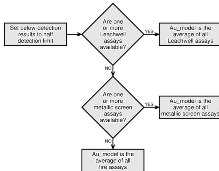
Figure 14-2 Assay selection hierarchy criteria at Castelo de Sonhos.
