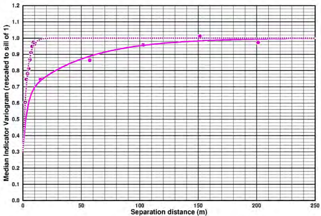
Figure 14-14 Median indicator variography for the surface enrichment layer, with the solid light purple line showing the omnidirectional variogram in the horizontal direction and the dotted darker purple line showing the variogram in the vertical direction.
