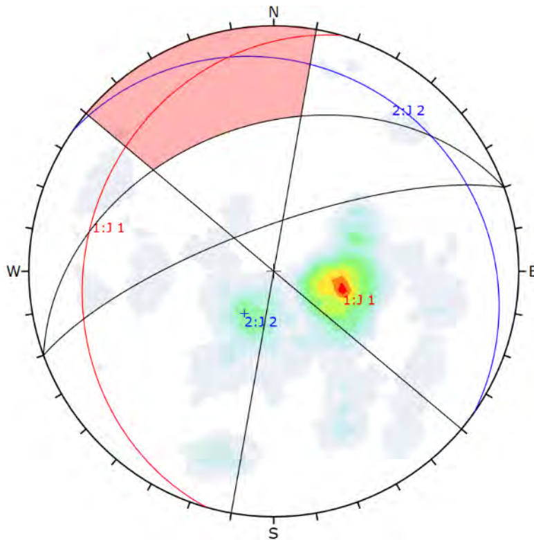
Figure 16-16 Kinematic analysis for the slope T2 showing 3% of probability for toppling rupture
