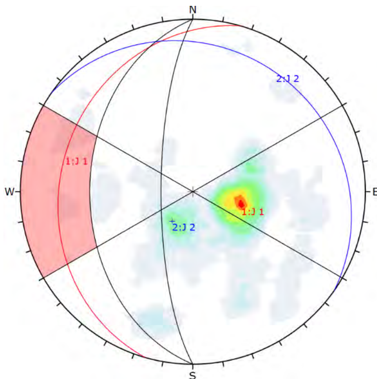
Figure 16-19 Kinematic analysis for the slope T3 showing 8% of probability for toppling rupture
