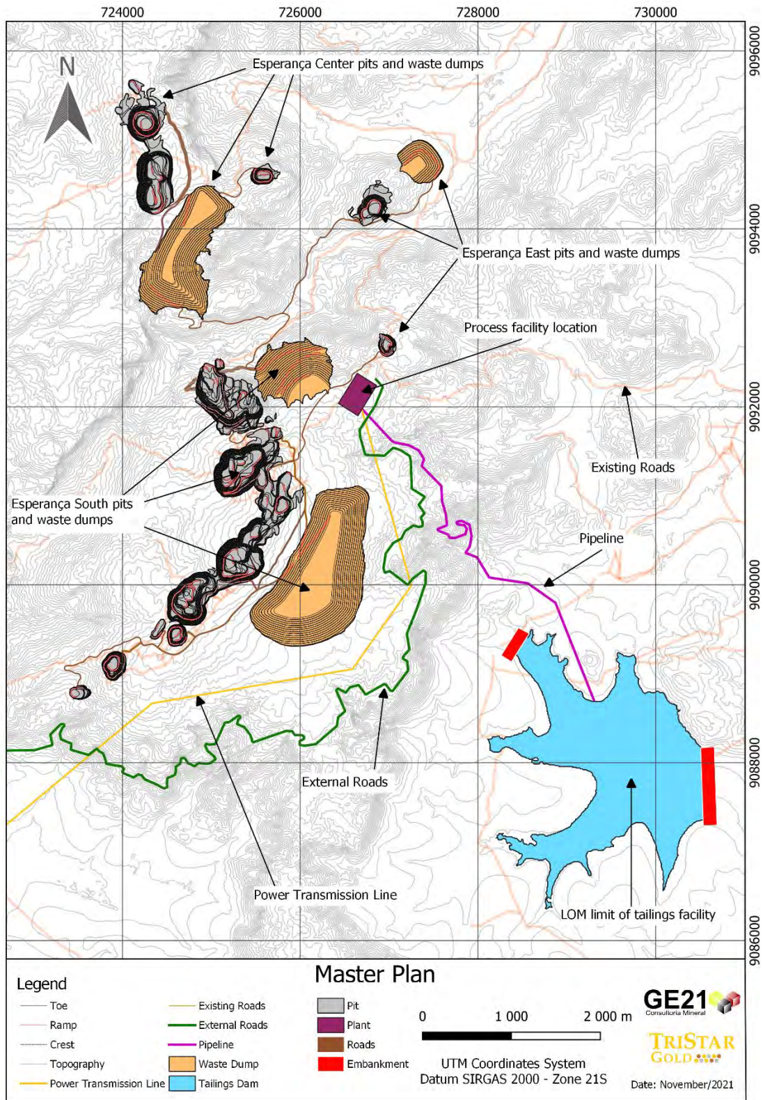
Figure 1-1: Project Layout
