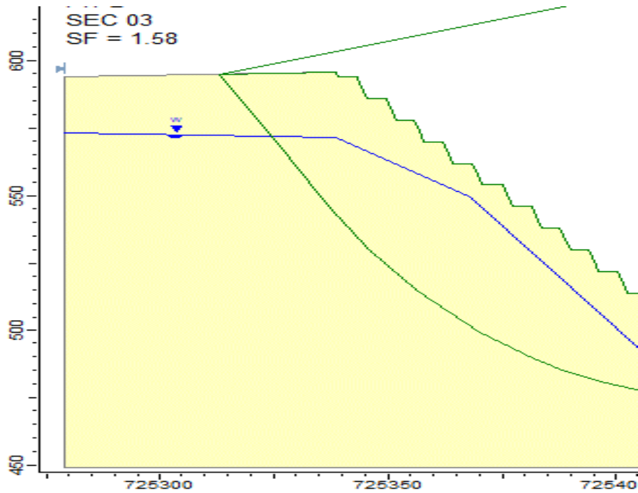
Figure 16-30 Limit-equilibrium analysis results for Section 03 with FS (security factor) = 1.58
