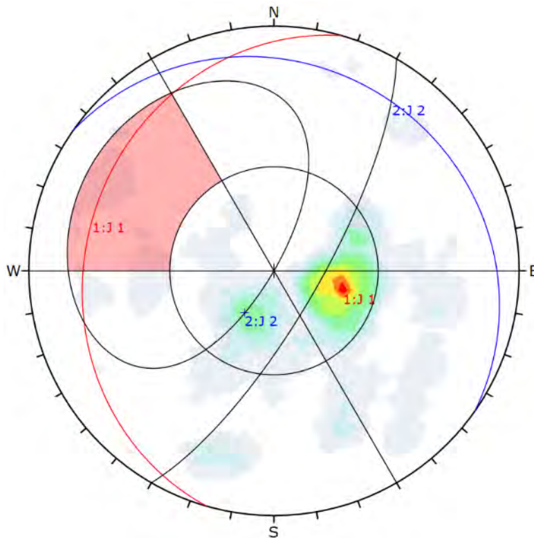
Figure 16-24 Kinematic analysis for the slope T4 showing 6% of probability for planar rupture
