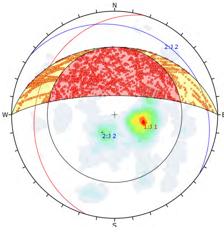
Figure 16-38 Kinematic analysis for the slope T7 showing 15% of probability for wedge rupture
