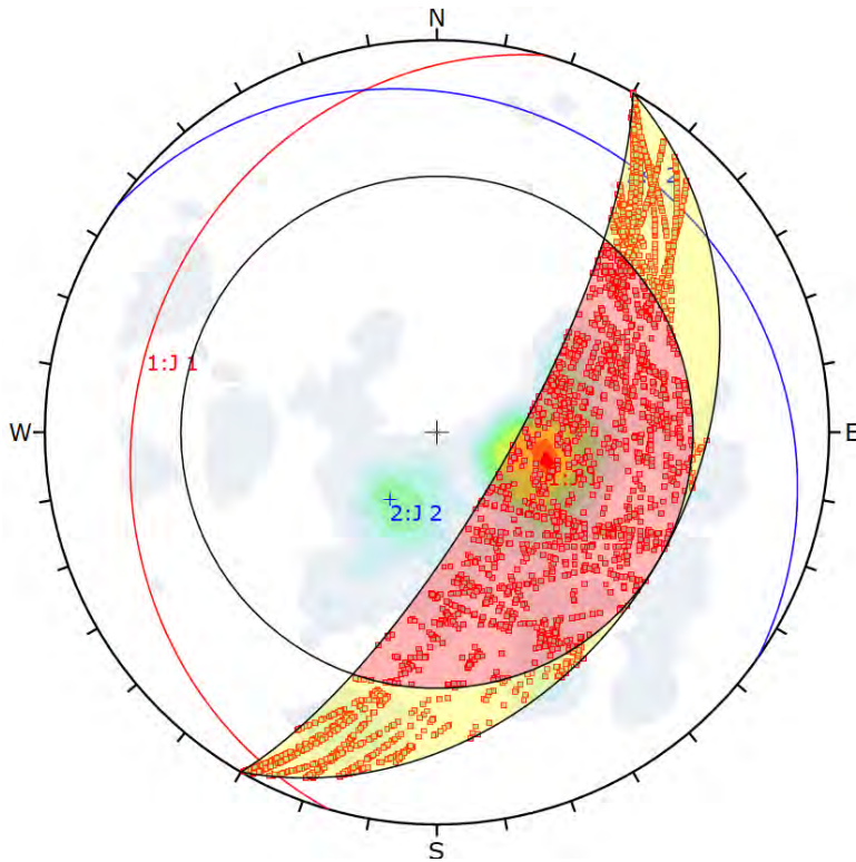
Figure 16-26 Kinematic analysis for the slope T4 showing 9% of probability for wedge rupture
