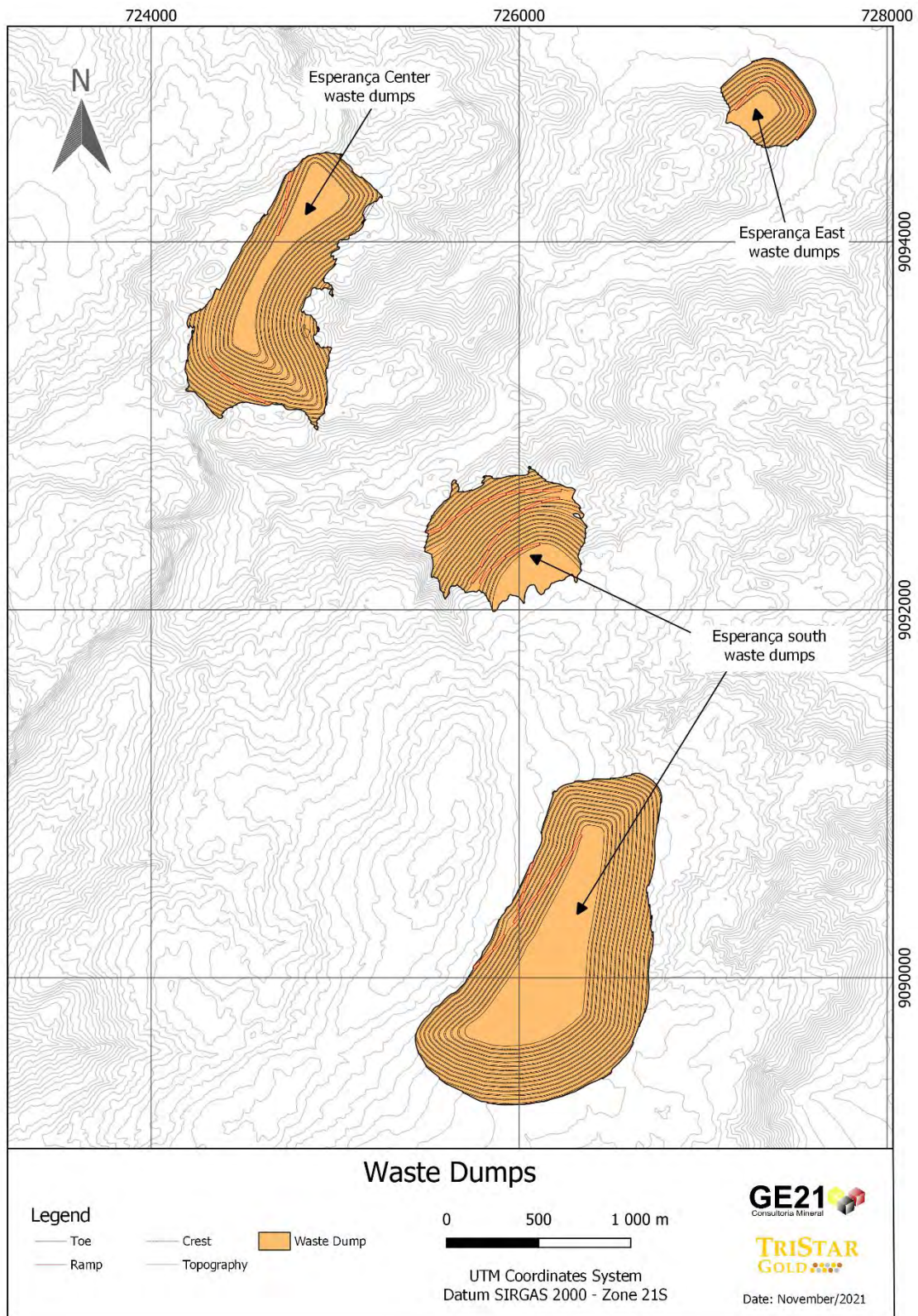
Figure 18-1 Waste Piles Layout for Castelo de Sonhos Project
