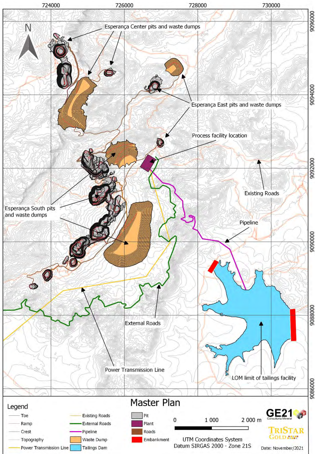
Figure 18-3 Project Layout
