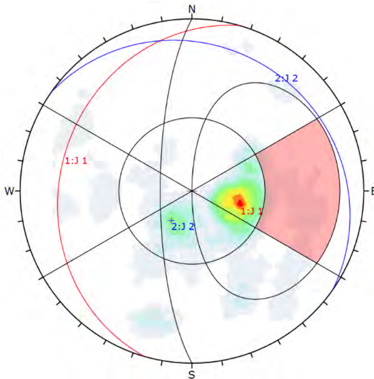
Figure 16-18 Kinematic analysis for the slope T3 showing 9% of probability for planar rupture
