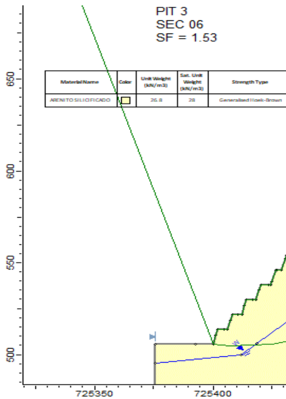
Figure 16-40 Limit-equilibrium analysis results for Section 06 with FS (safety factor) = 1.53
