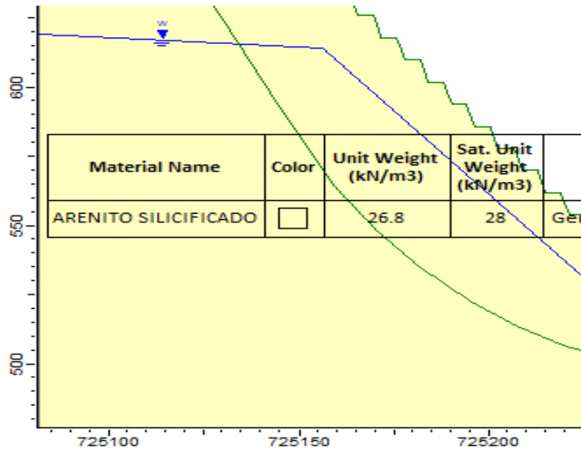
Figure 16-42 Limit-equilibrium analysis results for Section 08 with FS (safety factor) = 1.48
