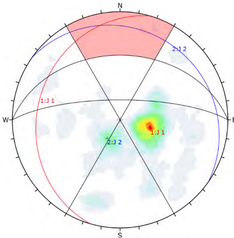
Figure 16-37 Kinematic analysis for the slope T7 showing 4% of probability for toppling rupture
