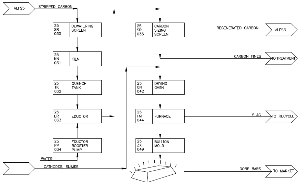
Figure 17-7 Simplified Conceptual Flowsheet – Carbon Regeneration and Smelting
